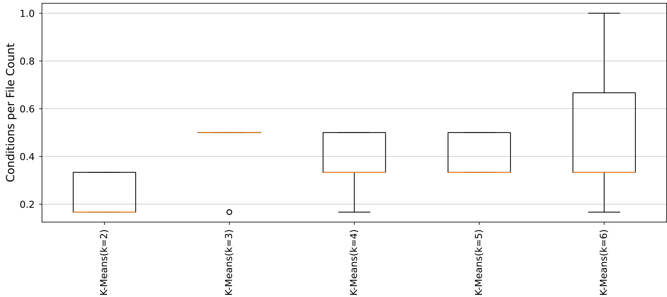
YARA Rules Conditions per File Count Distribution (Cluster23_Size6 dataset)
